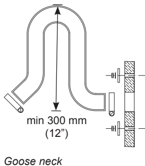
Goose neck
