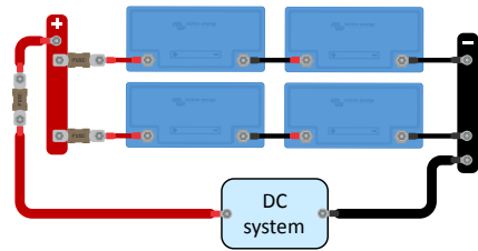
Meerdere accu's in serie / parallel
